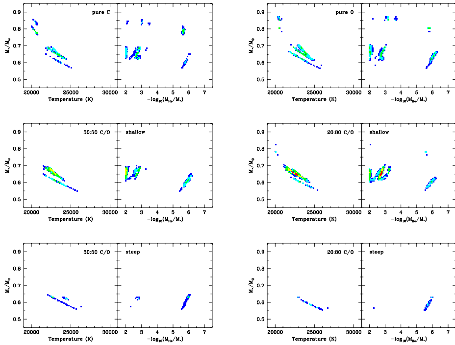
Figure 4.4: The families of models found by the GA which yield good matches to the periods observed in GD 358 for various core compositions and internal chemical profiles. The quality of the fit is indicated by the color of the square: r.m.s. < 3.0 seconds (blue), < 2.75 seconds (cyan), < 2.5 seconds (green), < 2.0 seconds (yellow), and < 1.65 seconds (red).
